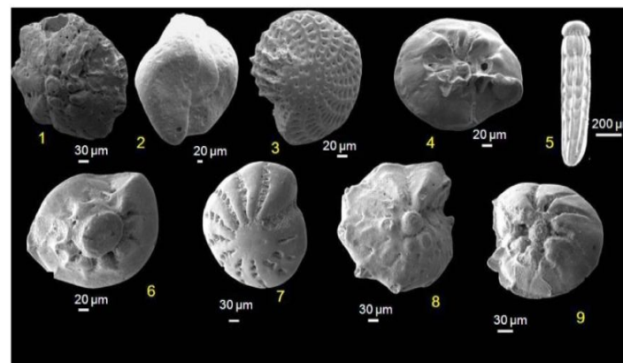
Fig. 15. Some of the selected species of foraminifera in Paleocene tsunami deposit I. 1. Calcarina sp., 2. Quinqueloculina sp., 3. Elphidium crispum , 4. Ammonia sp., 5. Rectobolivina raphanus , 6. Pararotalia sp., 7. Elphidium eichwaldi , 8. Calcarina calcar , 9. Ammonia sp.
